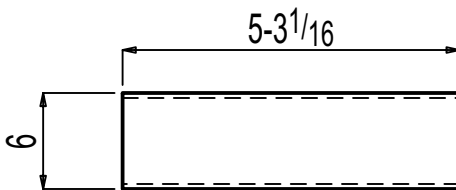
ONE HSS F-09.06M2
