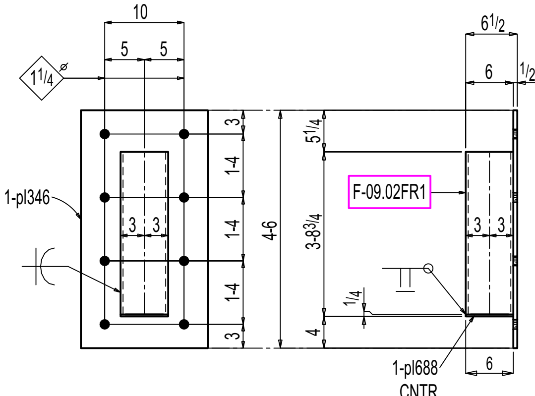
ONE FRAME F-09.02FR1
