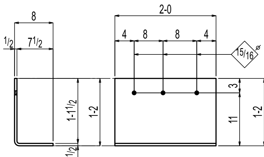
ONE BENT PLATE F-09.05BP1
