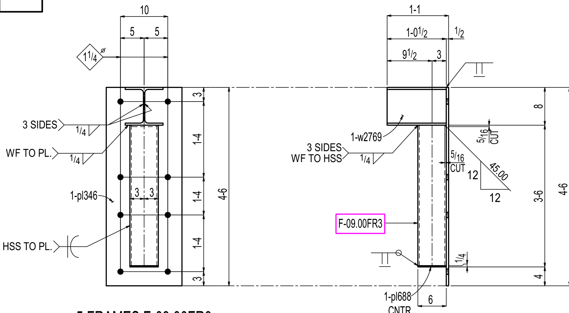
5 FRAMES F-09.00FR3
