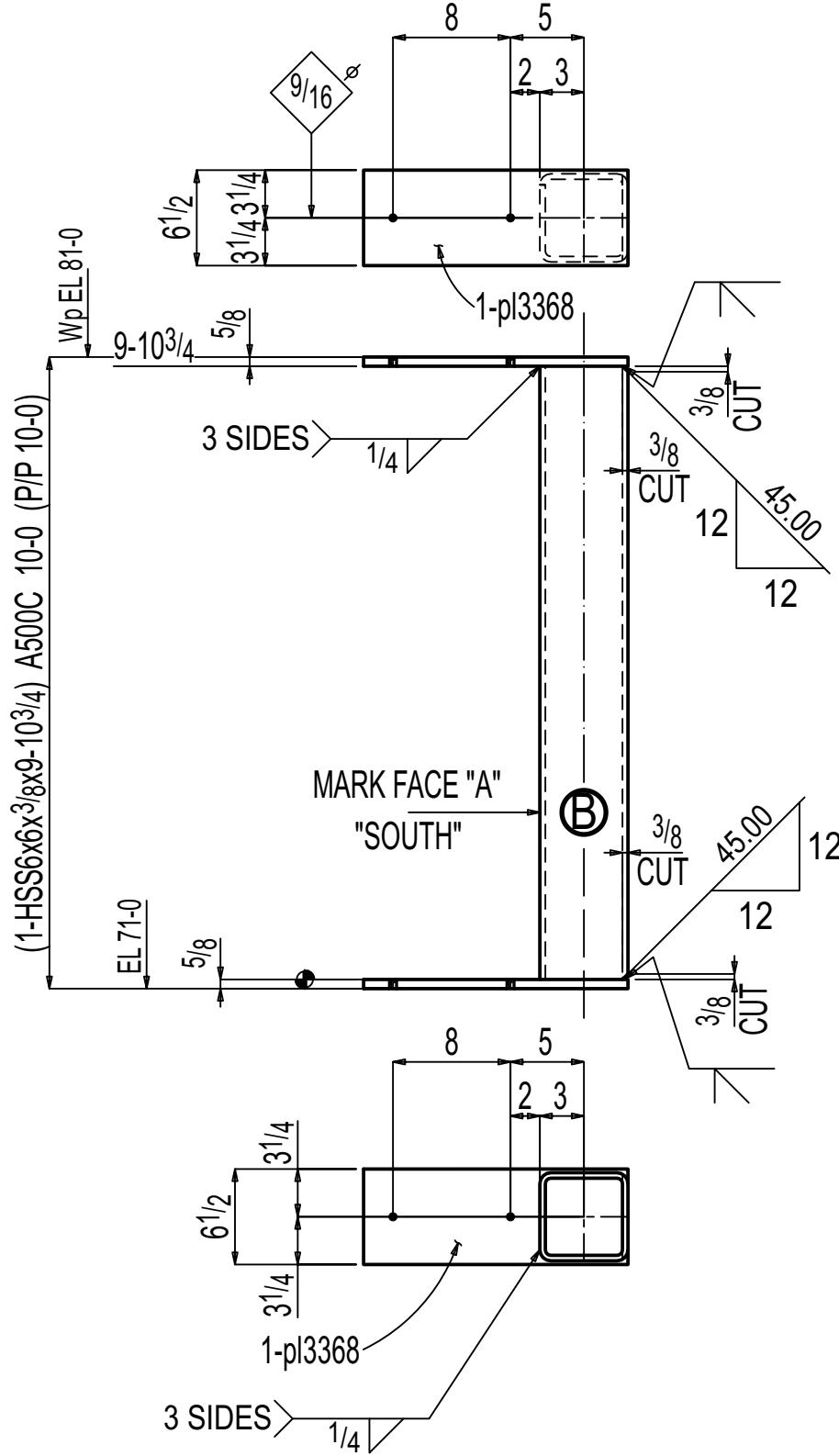
ONE COLUMN F-09.03C2
