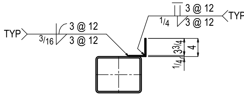
Section A-A F-09.03B2
