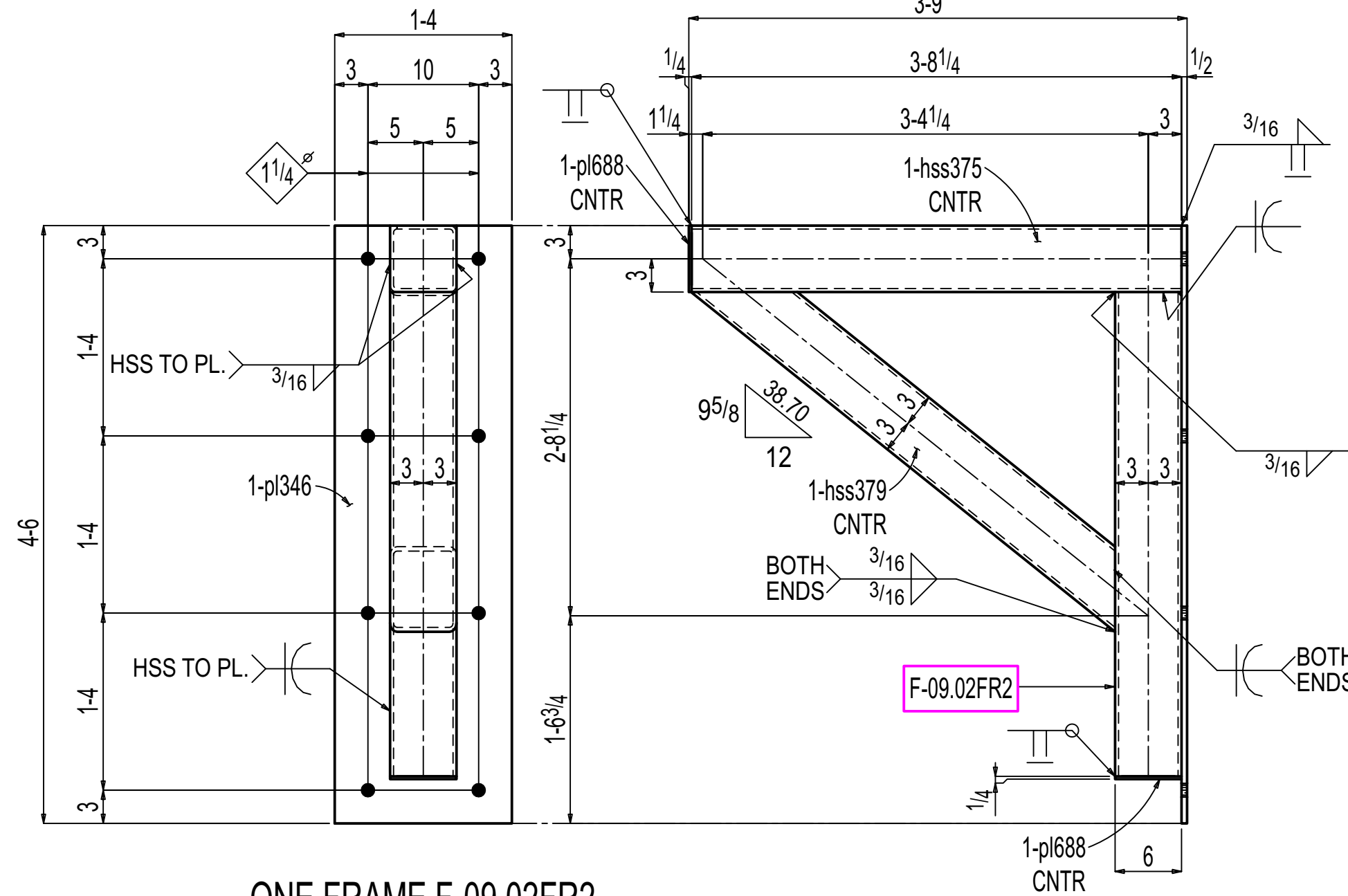
ONE FRAME F-09.02FR2
