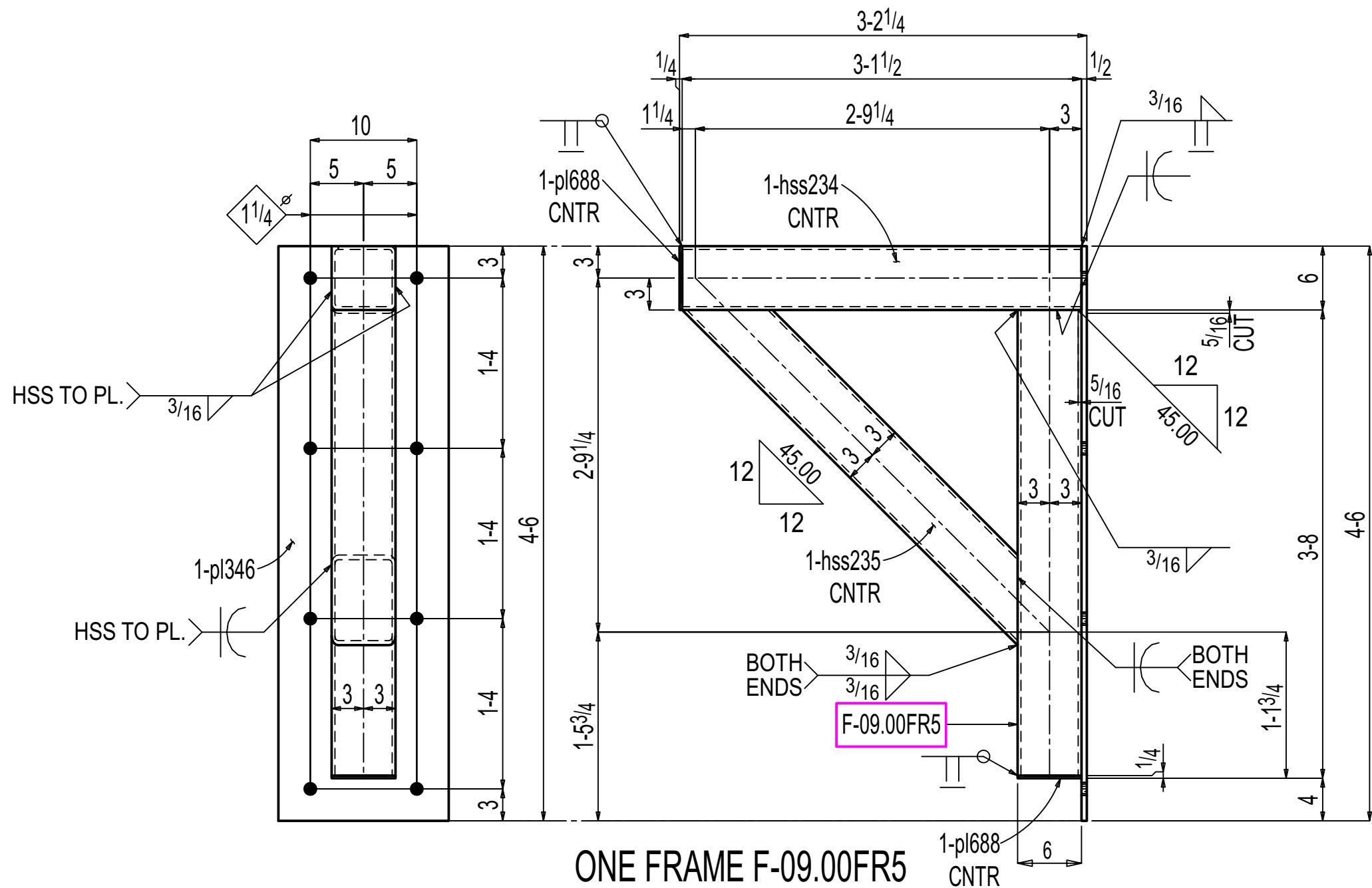
ONE FRAME F-09.00FR5
