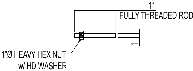
12 THREADED RODS F-09.05M10
