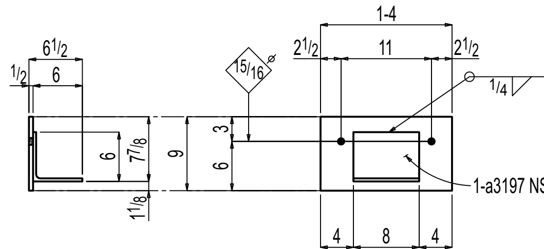
ONE PLATE F-09.02M6
