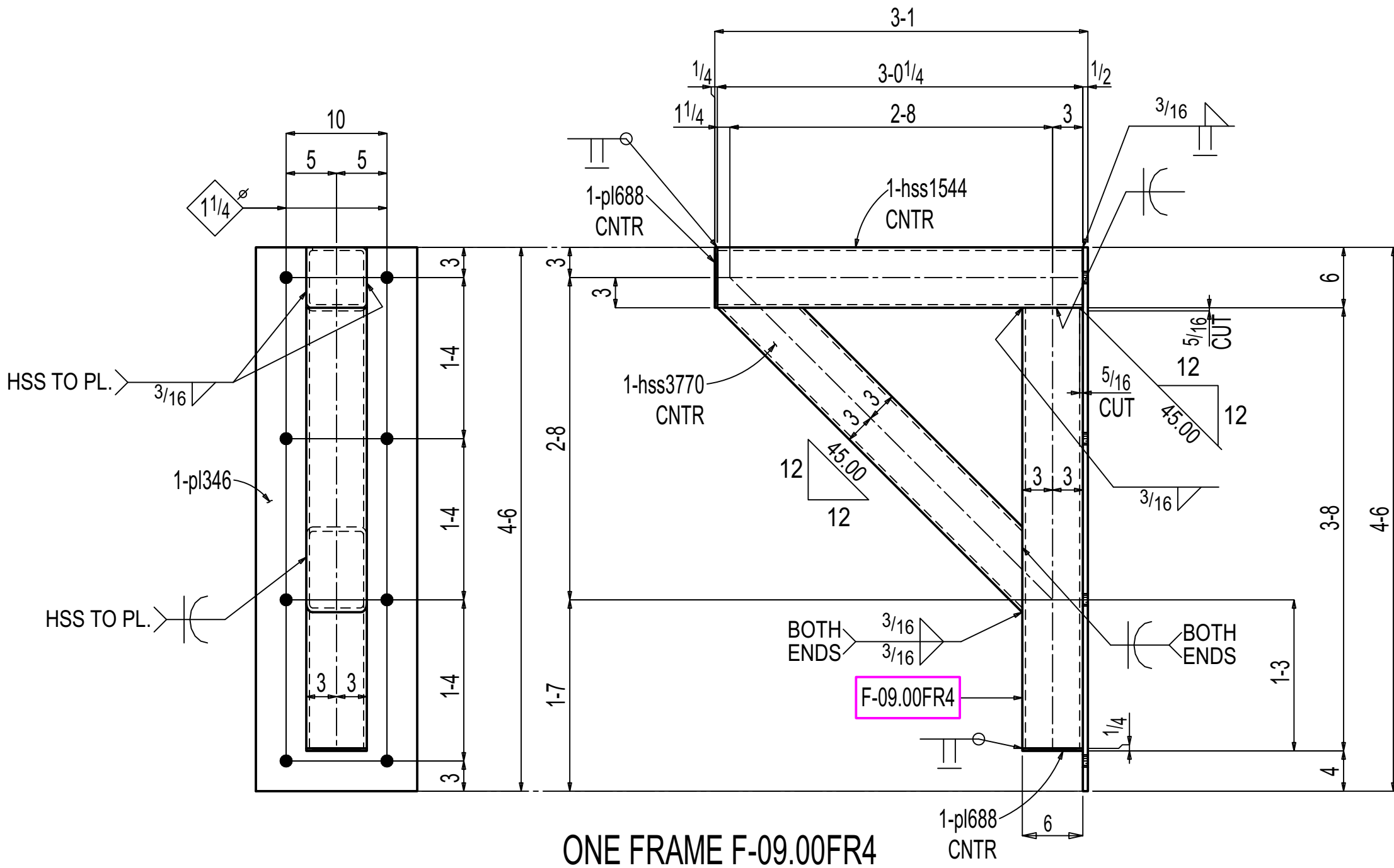
ONE FRAME F-09.00FR4
