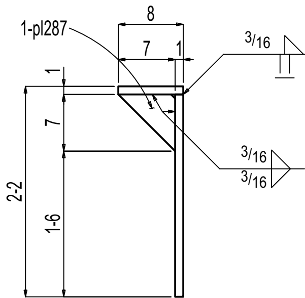
Section A-A F-09.02M1
