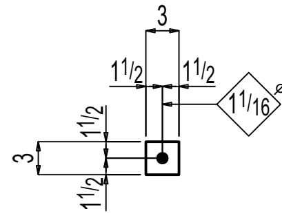
6 PLATE WASHERS F-09.05M7
