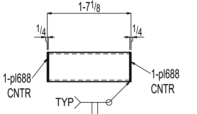
ONE HSS F-09.05M3
