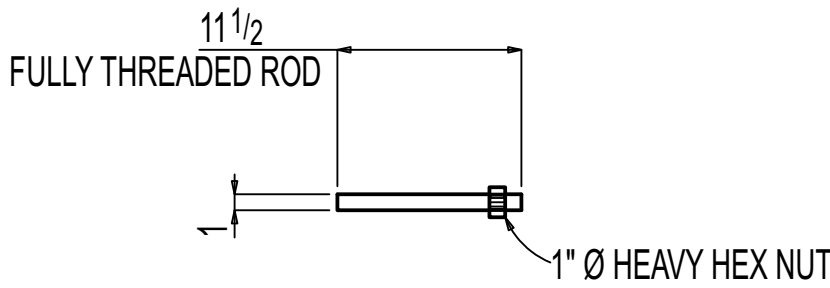
6 THREADED RODS F-09.05M8
