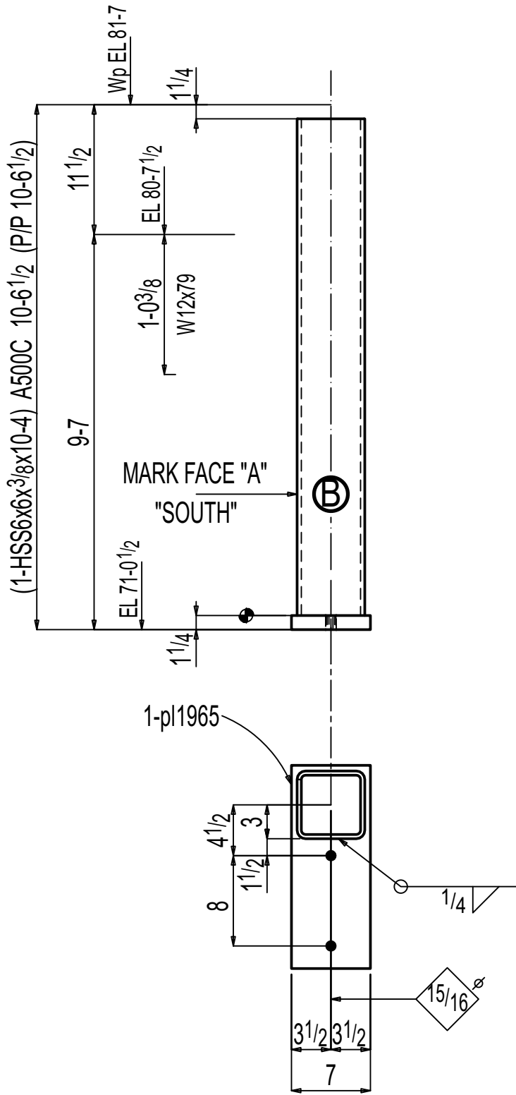
ONE COLUMN F-09.03C1
