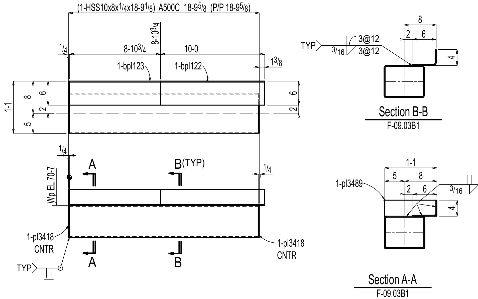
ONE BEAM F-09.03B1
