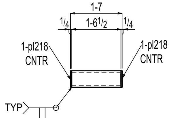
2 HSES F-09.05M2
