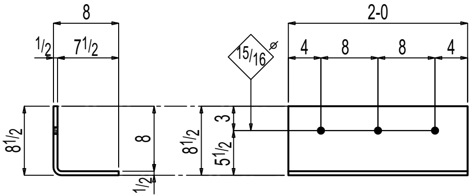
ONE BENT PLATE F-09.05BP2
