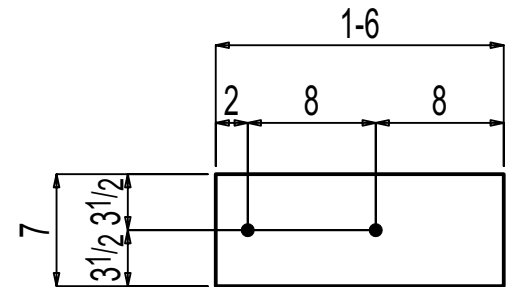
ONE LEVELING PLATE F-10.03LP2
