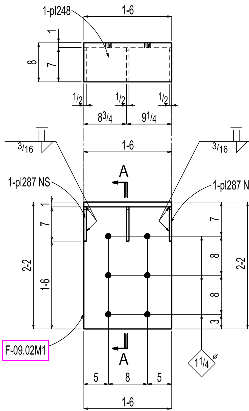
ONE PLATE F-09.02M1
