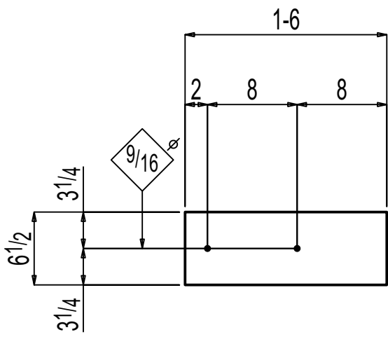
ONE LEVELING PLATE F-09.05LP1
