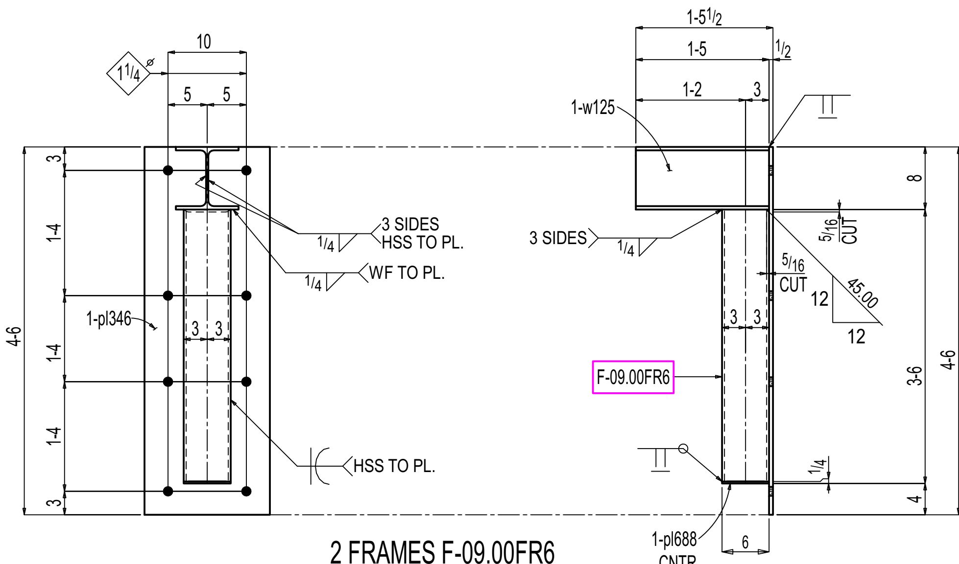
2 FRAMES F-09.00FR6
